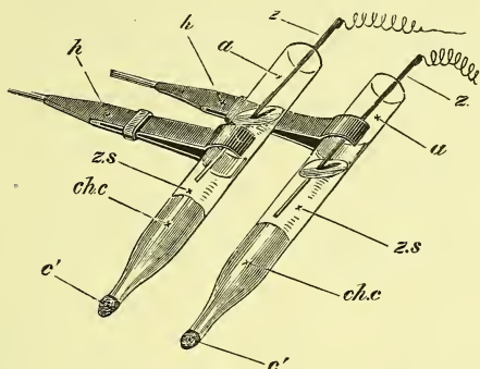
FIG. 18. NON-POLARISABLE ELECTRODES.
